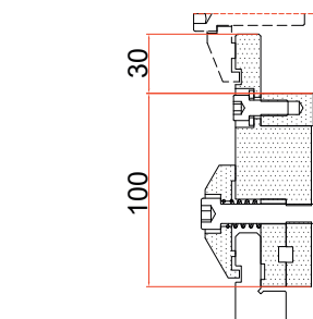
Euro American Type Mechanical Punch Clamping
