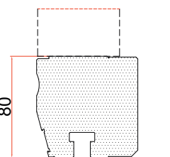
Wila American Type Hydraulic Punch Clamping
