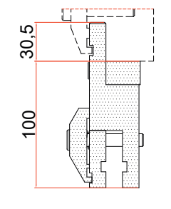
American Type Mechanical Punch Clamping
