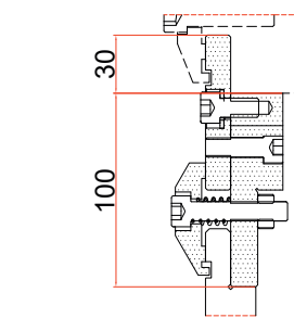
Euro Type Mechanical Punch Clamping
