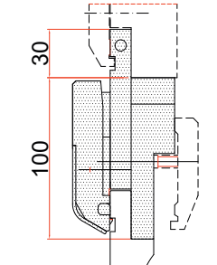
Euro Type Pneumatic Punch Clamping
