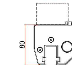
Wilson Hydraulic Automatic Punch Clamping
